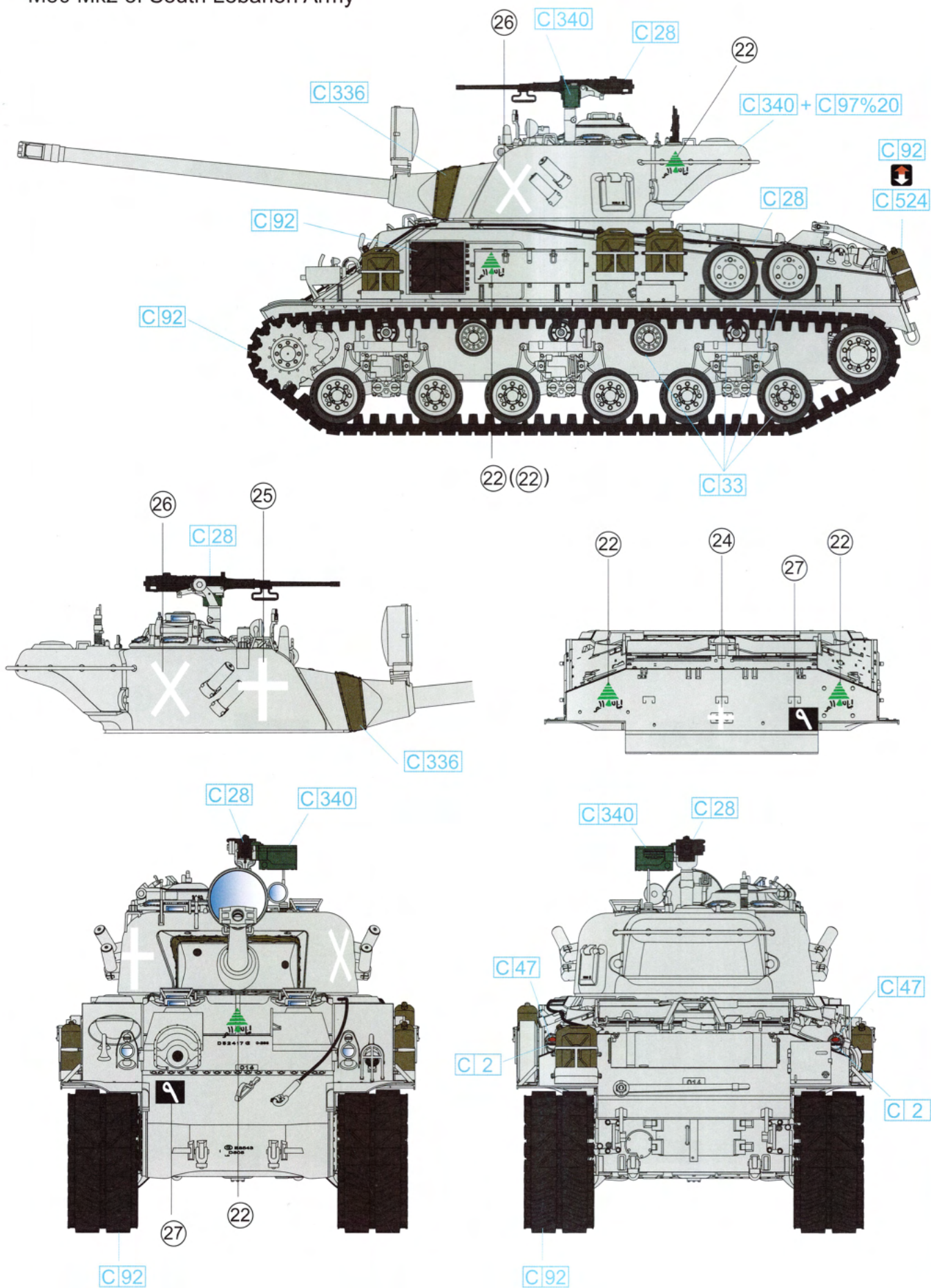
南黎巴嫩军的M50 Mk2 M50 Mk2 of South Lebanon Army
